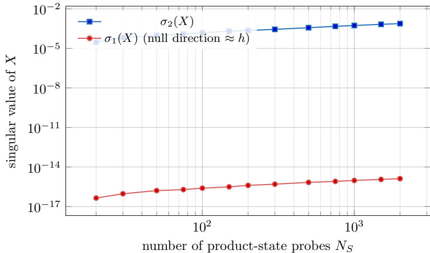
Open-boundary TFIM, n = 10 , t = 400
